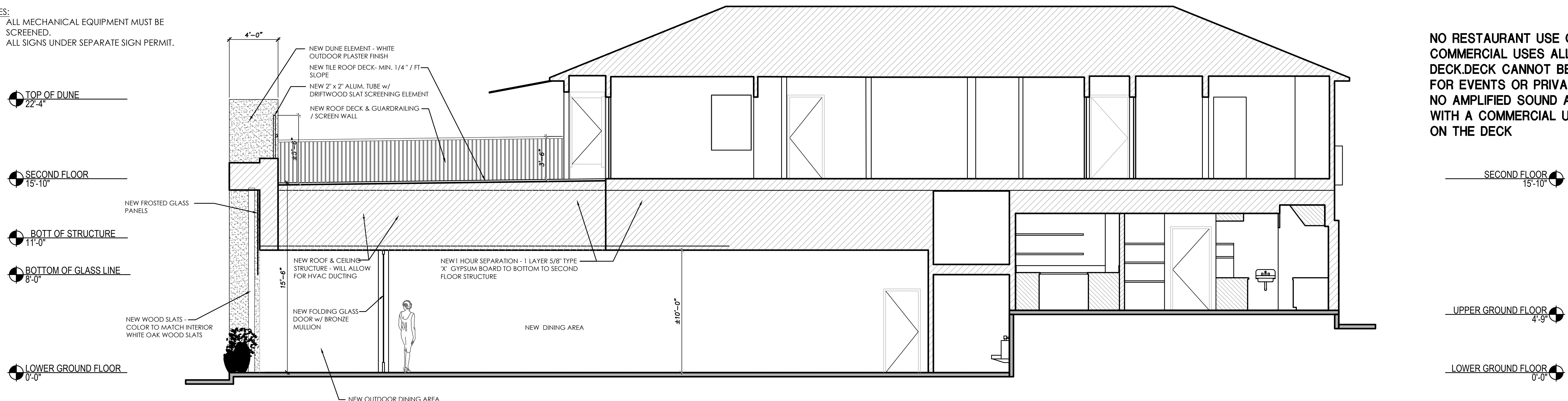
BUILDING SECTION 1/4"=1'-0" 1
