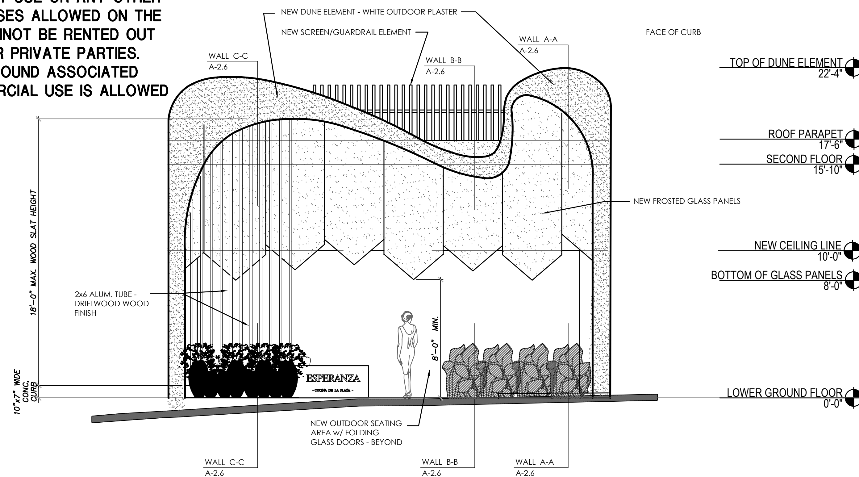
NEW ENTRY ELEVATION 1/4"=1'-0" 3
