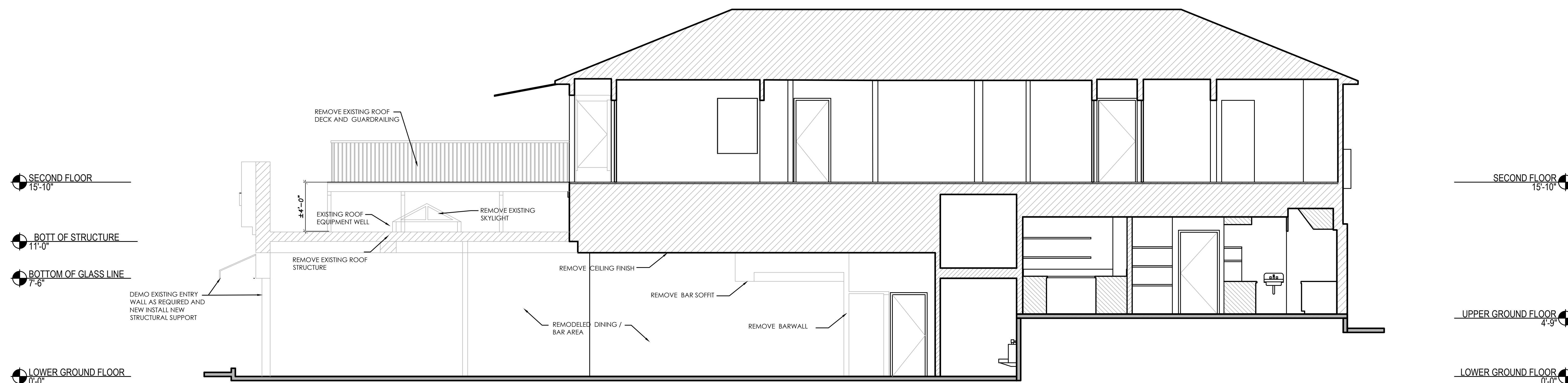
DEMO ENTRY ELEVATION 1/4"=1'-0" 4
