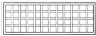
STANDARD SQUARE LATTICE
