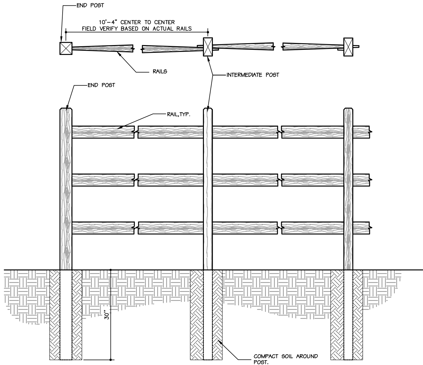
Split rail fence detail
