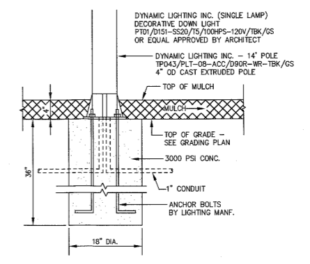
H15 1651LD04 AREA POST LIGHT DETAIL NTS
